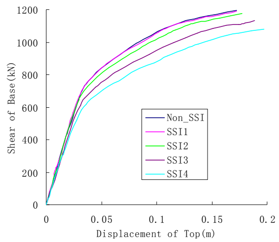
Figure 4.2 Relationship between structural base shear and top lateral displacement
