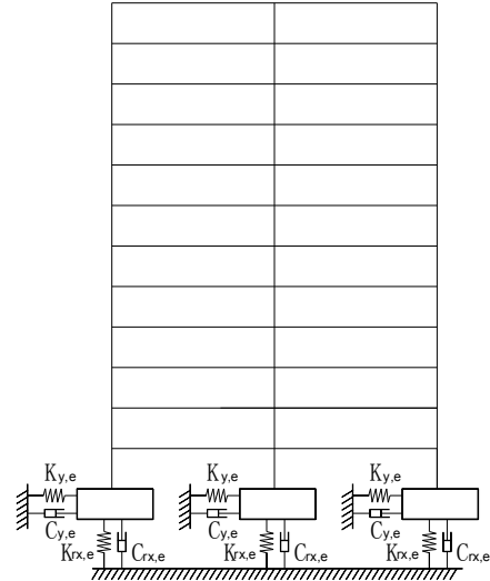
Figure 3.1 simplified model of soil-frame structure interaction system
