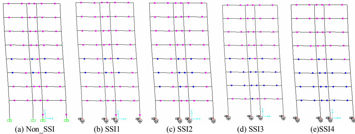
Figure 4.4 Distribution of plastic hinges
