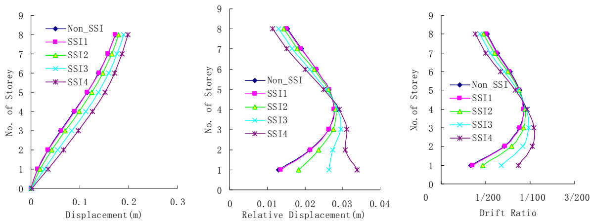
Figure 4.3 floor displacement and inter-story drift
