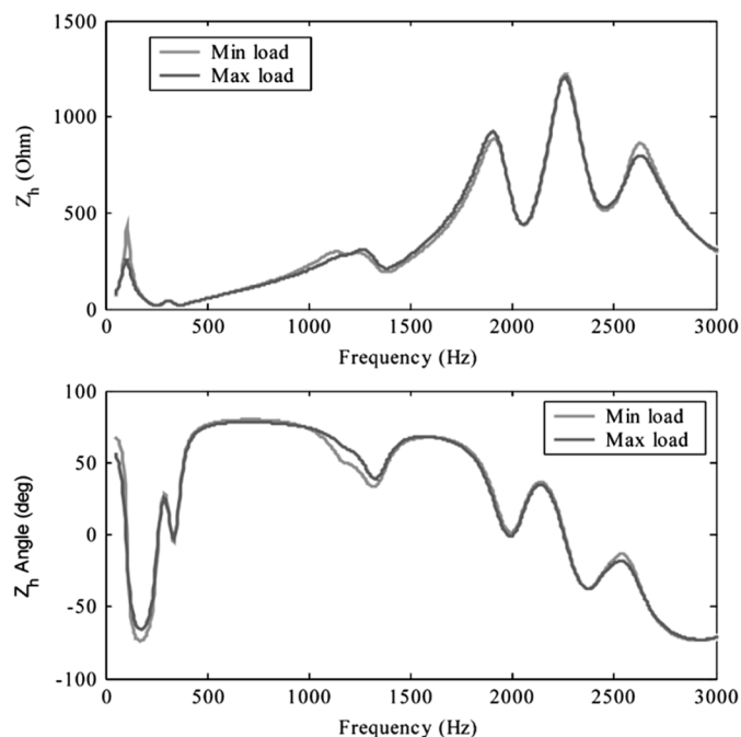
Fig. 6. Magnitude and angle of the harmonic impedance at the 150-kV busbars of Argostoli, for maximum and minimum load conditions.
