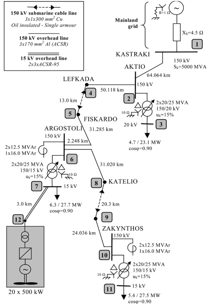
Fig. 3. One-line diagram of the study case system.
