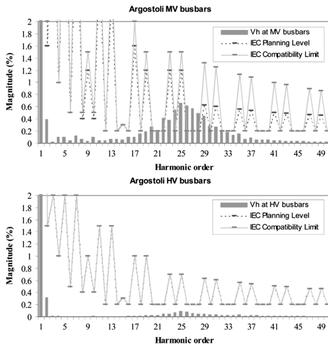
Fig. 12. Voltage distortion per harmonic order at the MV and HV busbars of Argostoli, for minimum load conditions, calculated with the simplified MV network model.
