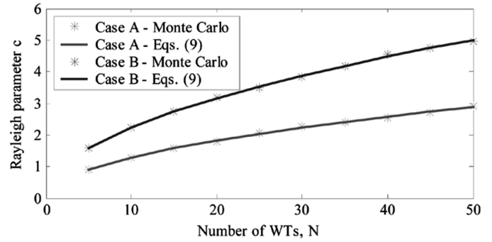
Fig. 21. Parameter c of the Rayleigh pdf of the wind farm harmonic current magnitude, calculated from the Monte Carlo simulation results and from the empirical (9), for Cases A and B.
