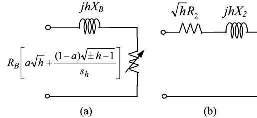
Fig. 2. (a) Induction and (b) synchronous machine harmonic equivalents.
