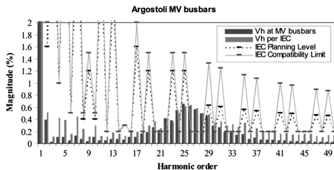
Fig. 18. Calculated voltage harmonics at the Argostoli MV busbars using the simplified method and from the harmonic load flow (Fig. 12).
