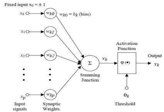
Fig 5 Mathematical model of neural network
