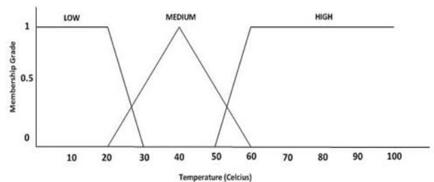
Figure 4: Membership degrees for temperature
